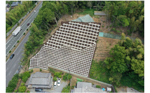
Toko Geotech Mii School district Slope countermeasure construction
